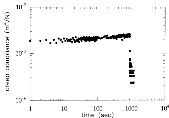
Fig. 10. Creep experiment on a methylcellulose solution stabilized for 2 h at 65°C (solvent: water, c = 15 g/l).
